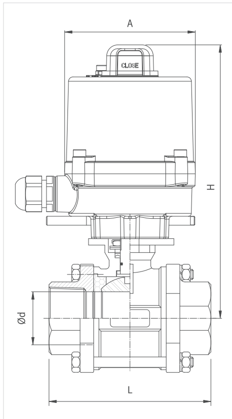
Dimensions (3-Piece)
